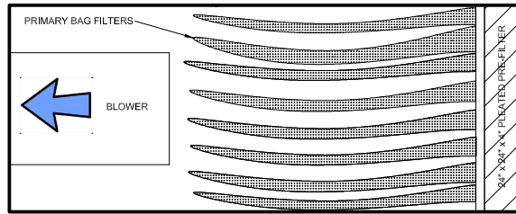
TOP VIEW : CUT-AWAY
